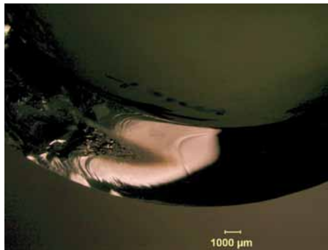
Figure 4. The fracture surface of a soda lime silicate glass cookware bowl (from bowl in Figure 3) as it formed during thermal shock failure. Note the Wallner lines trailing along the surfaces, inside and out, are indicative of heat strengthening of the glass during manufacturing. 22
